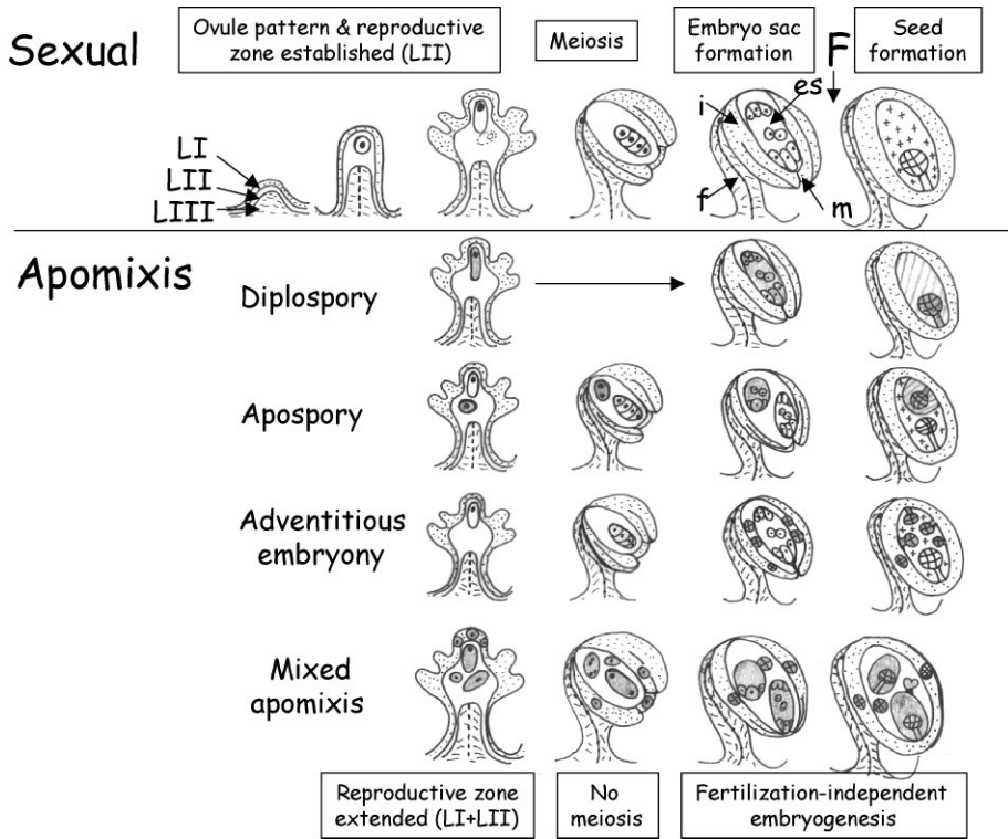
Figure 1 Sexual and apomictic reproduction in the ovule of flowering plants. The cartoon summarizes ovule development beginning with the formation of the primordium made up of the LI, LII, and LIII layers. The events of sexual reproduction are displayed in the top panel above the line. Apomictic processes are shown below the line and cells or structures involved in apomixis are shaded in grey while those pertaining to sexual reproduction remain white. Abbreviations: a, archesporial cell; e, embryo, en, endosperm; es, embryo sac; f, funiculus; F, double fertilization, i, integuments; m, micropyle; mmc, megaspore mother cell.
