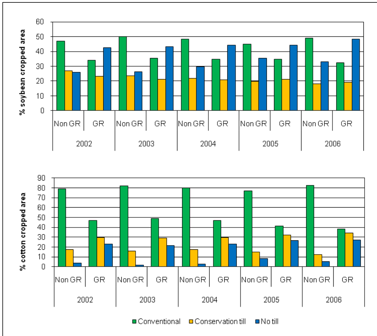
Figure 3. Comparison of US tillage practices in glyphosate-resistant (GR) and non-GR soybean (top) and cotton (bottom) from 2002 through 2006 as a percentage of hectares planted. Used with permission from Dill et al. (2008).
