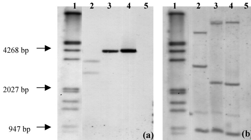
Fig. 2. Southern analyses of DNA from selected transgenic PAR plants digested with EcoRV : (a) DNA was probed with nptII and (b) DNA was probed with uidA . Lane 1: DIG-labeled DNA molecular weight marker III (Roche); lane 2: PAR 65; lane 3: PAR 66; lane 4: PAR 68; lane 5: control DNA from an untransformed plant.
