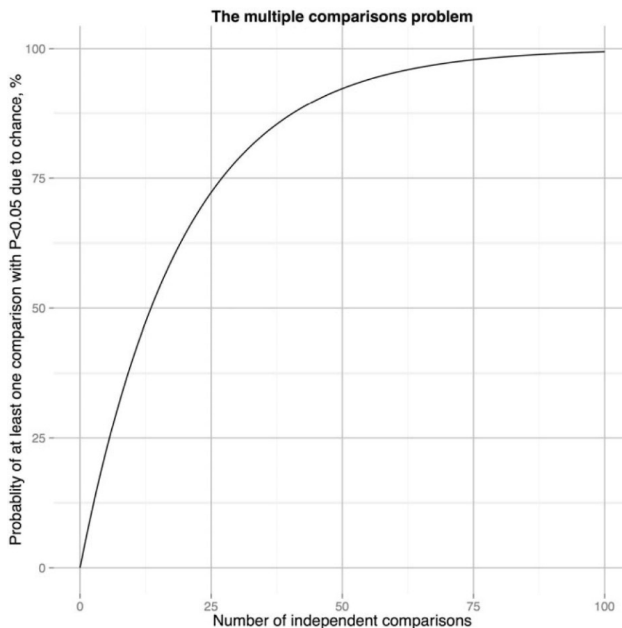
Figure 1. The problem of multiple comparisons. The probability of at least one “significant” comparison is computed from the number of comparisons (N) using the following equation: (1.00 - 0.95^N) \times 100\% .
